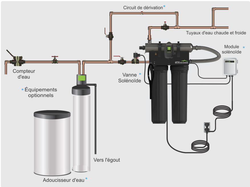
Figure 1. Installation Typique
